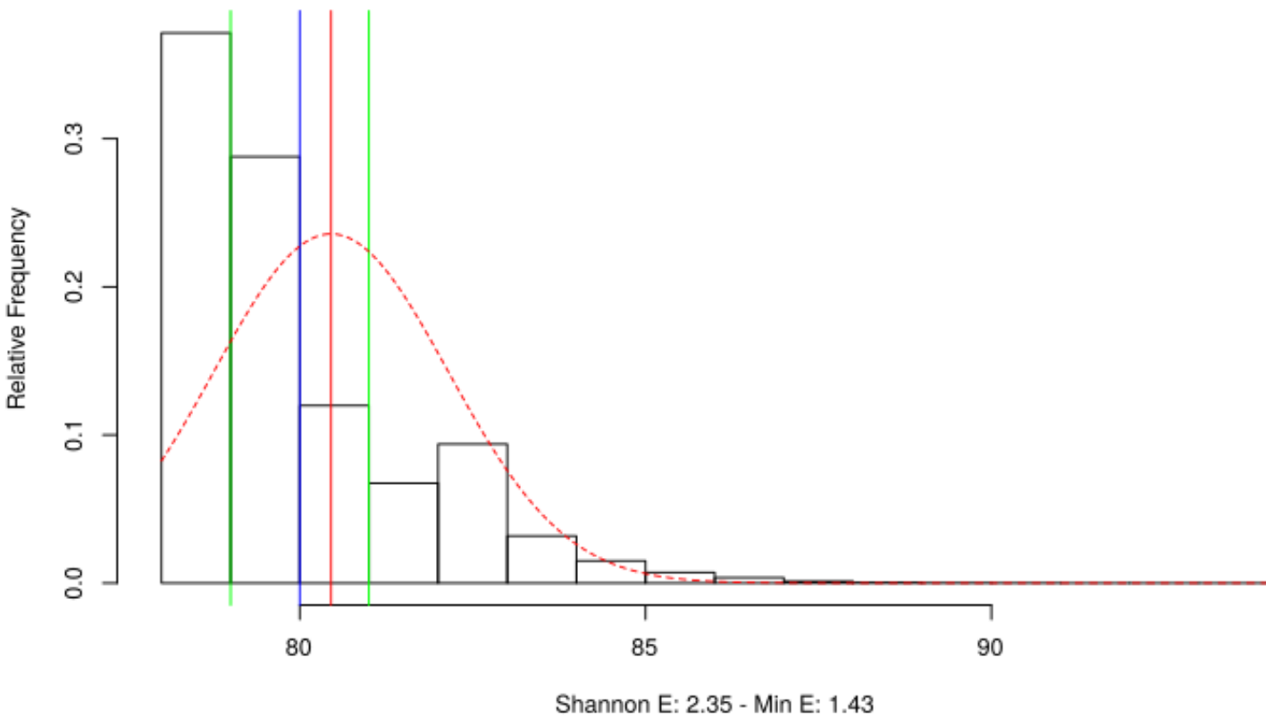
Distribution of time delta in A10_jitterentropy_lfsrtime.out up to 95 (single)
