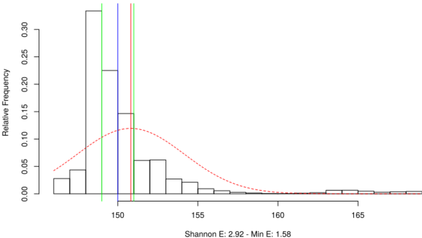
Distribution of time delta in A7_jitterentropy_lfsrtime.out up to 170 (single)
