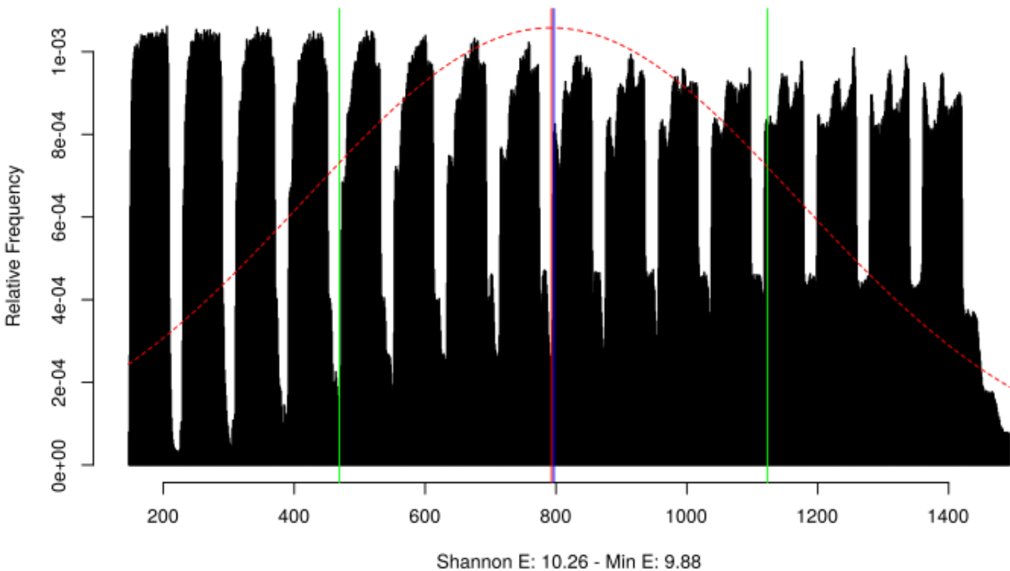
Distribution of time delta in A7_jitterentropy_lfsrtime.out up to 1495 (varying)
