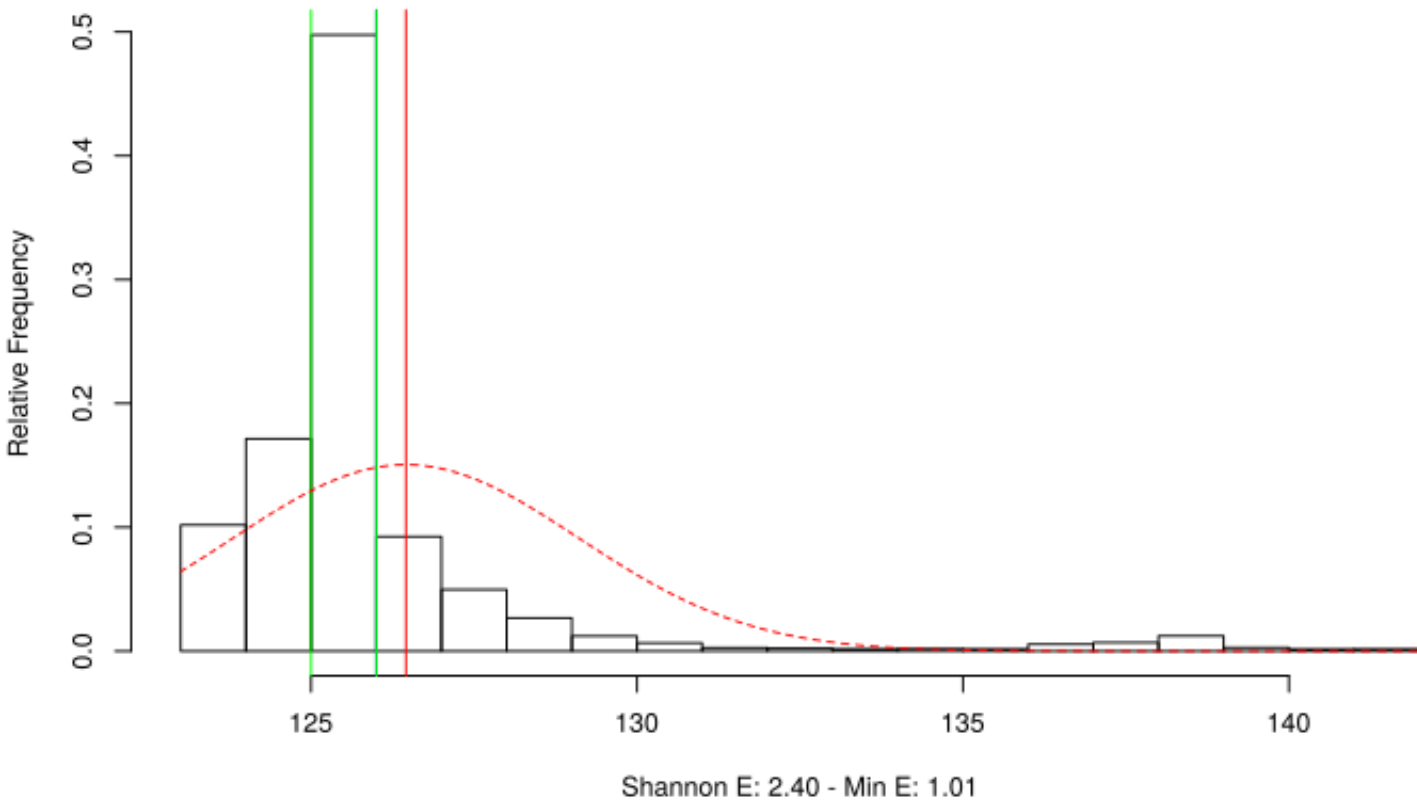
Distribution of time delta in A8X_jitterentropy_lfsrtime.out up to 143 (single)
