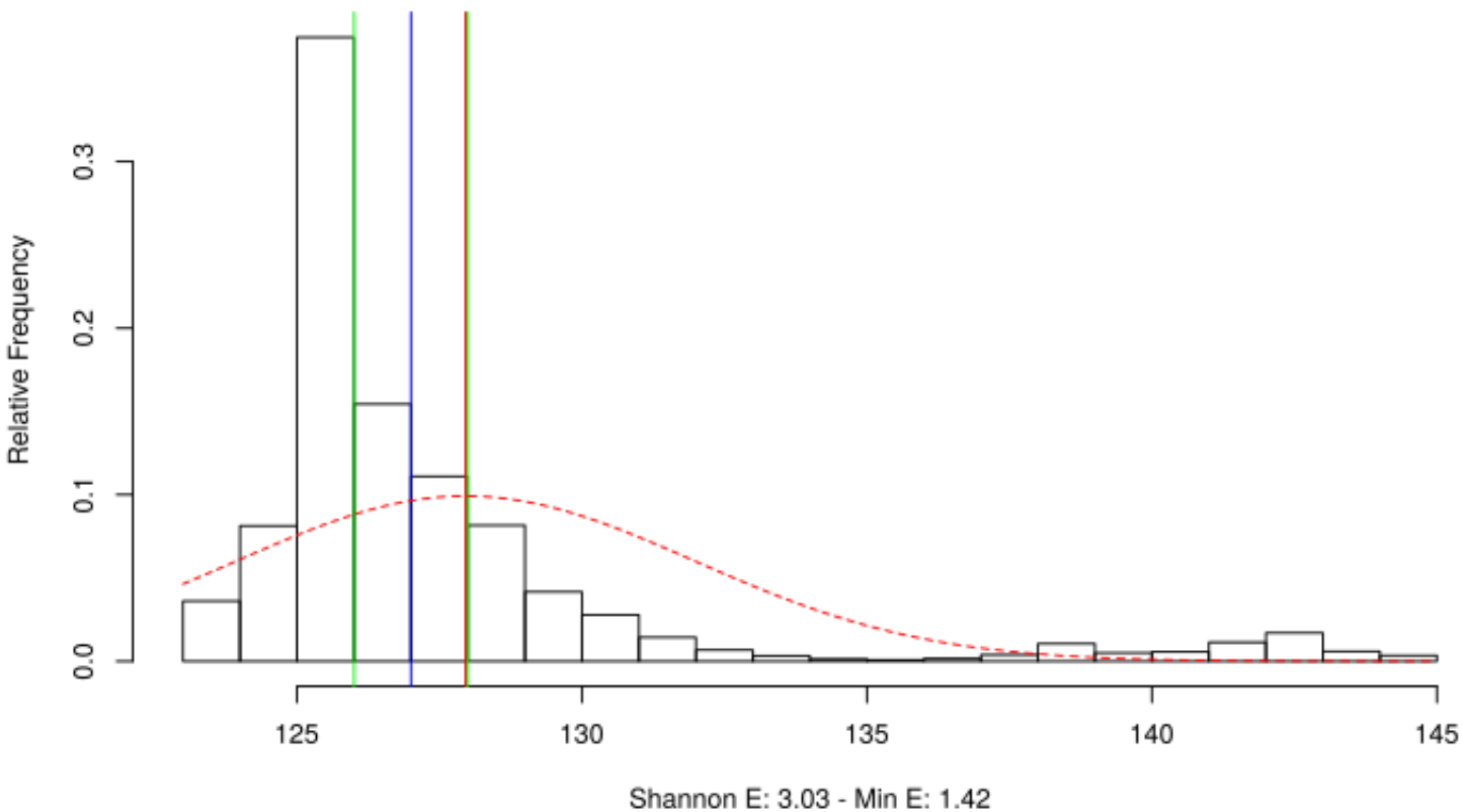
Distribution of time delta in A8_jitterentropy_lfsrtime.out up to 146 (single)
