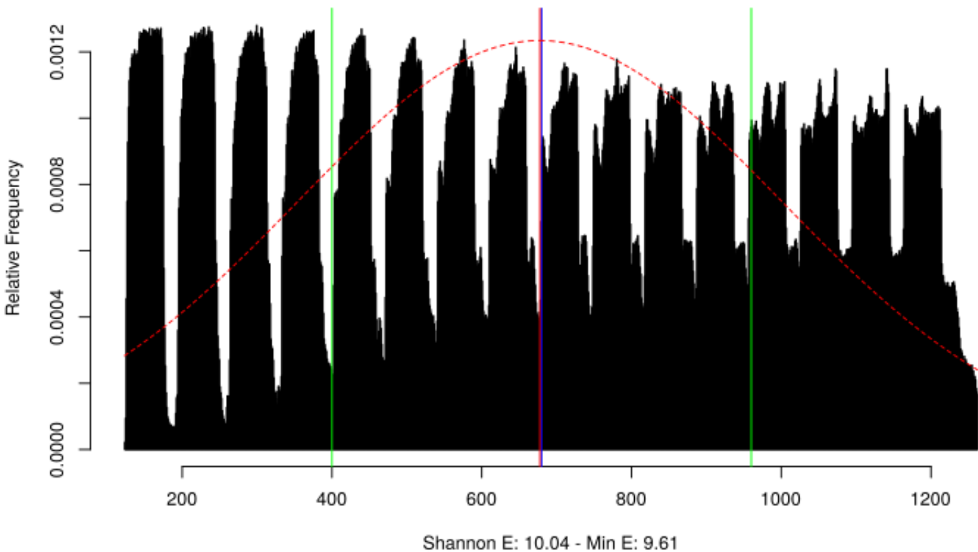
Distribution of time delta in A8_jitterentropy_lfsrtime.out up to 1264 (varying)
