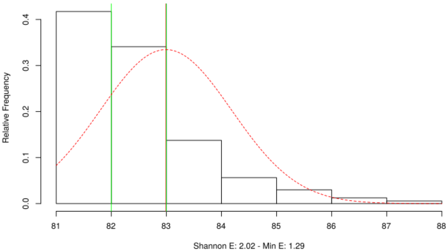
Distribution of time delta in A9X-jitterentropy_lfsrtime.out up to 89 (single)
