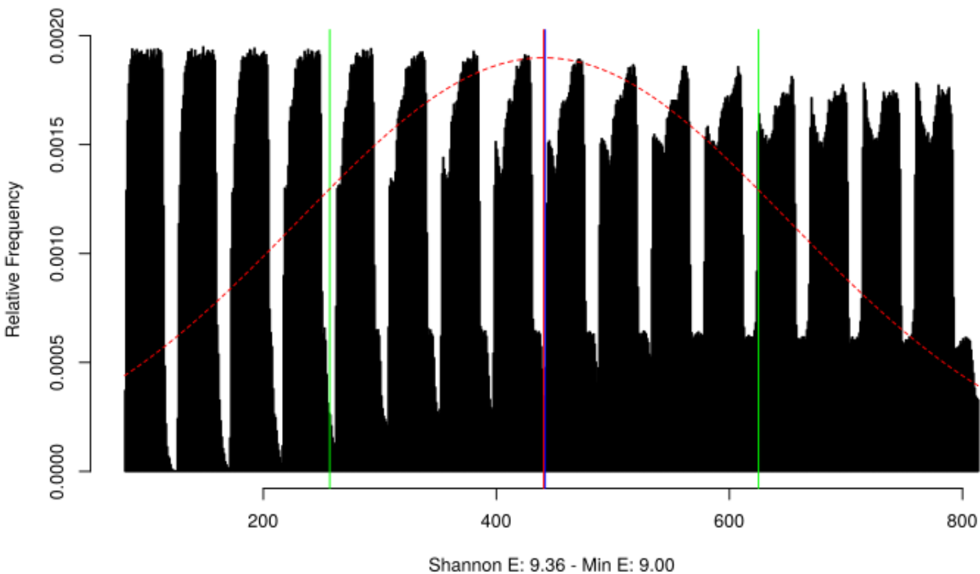
Distribution of time delta in A9X-jitterentropy_lfsrtime.out up to 815 (varying)
