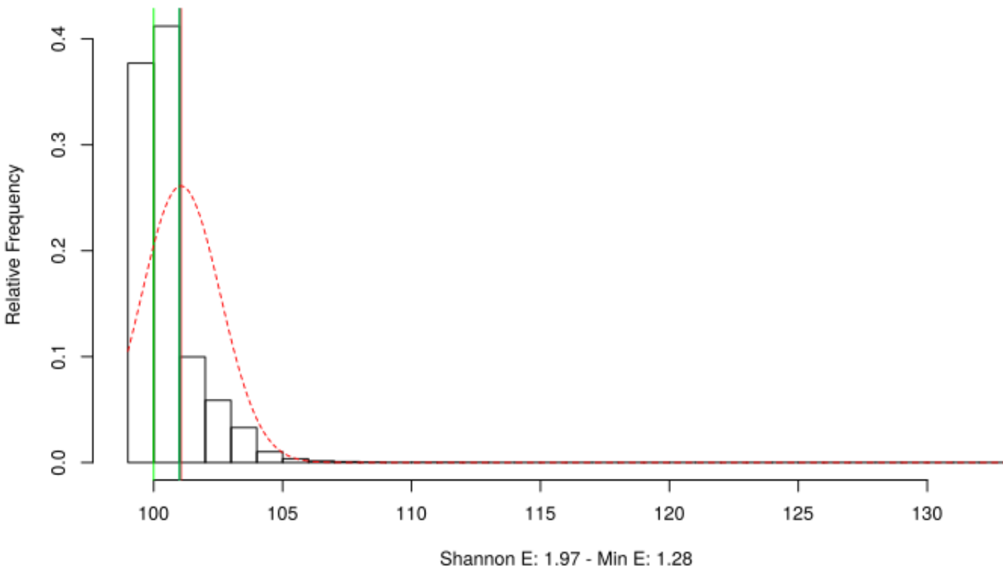
Distribution of time delta in A9_jitterentropy_lfsrtime.out up to 134 (single)
