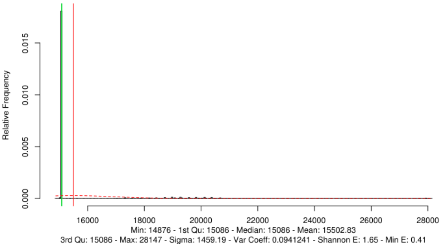
Distribution of time delta in userspace-foldtime-atomz530.varmemaccess.O0.data up to 28216 (sing
