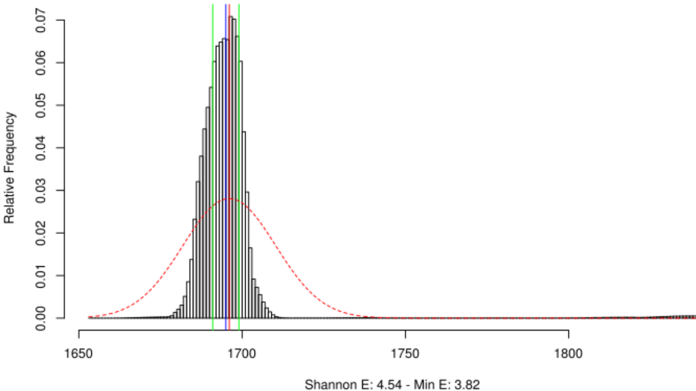
Distribution of time delta in userspace-foldtime-i7-5557U.O0.data up to 1840 (single)
