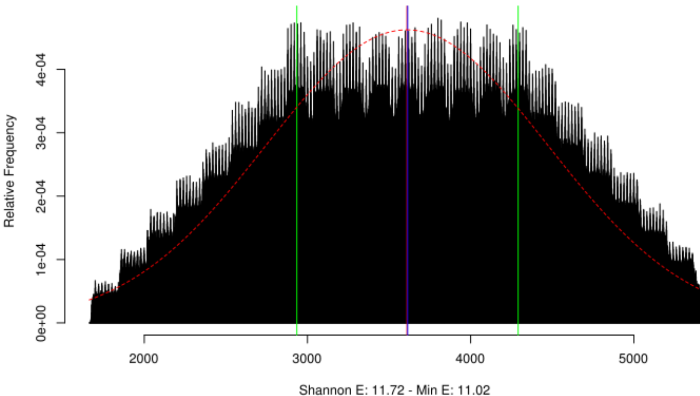
Distribution of time delta in userspace-foldtime-i7-5557U.O0.data up to 5413 (varying)
