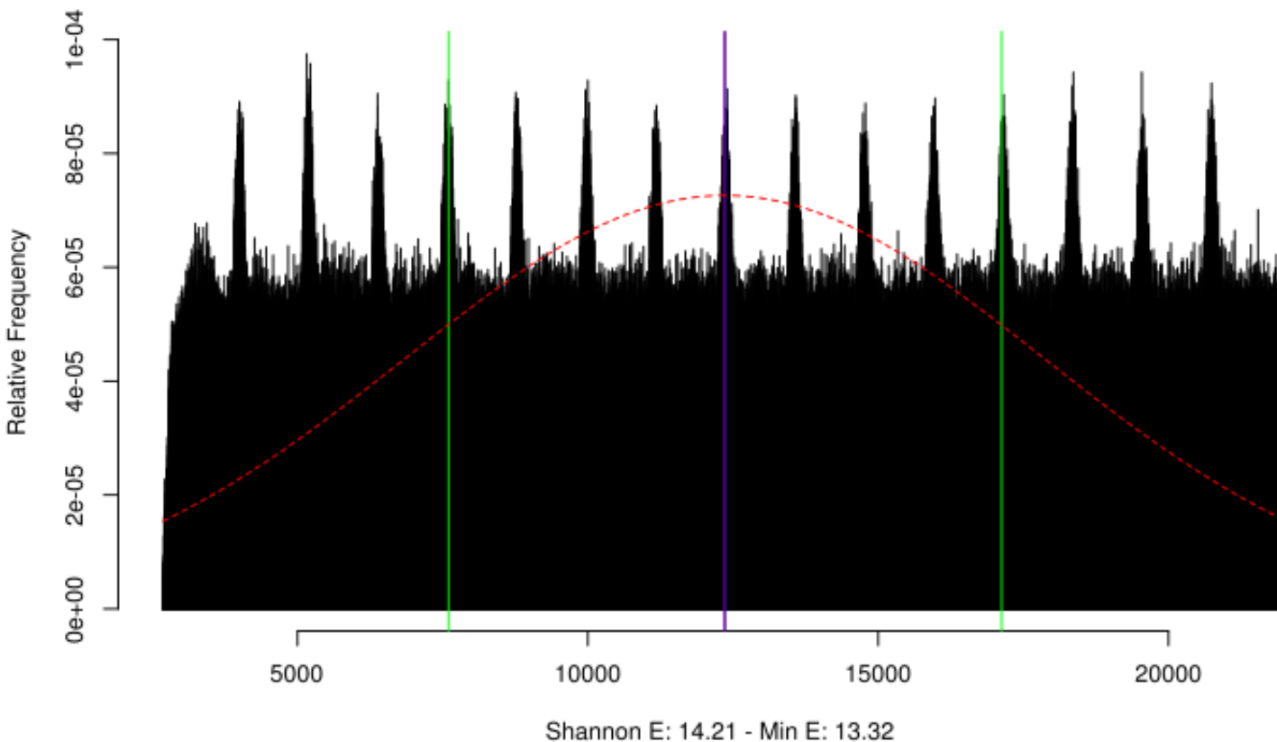
Distribution of time delta in userspace-foldtime-v2.0-i7-5557U.O0.data up to 21904 (varying)
